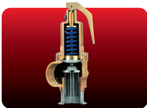
Fig. 500SS Pressure Relief Valve with Stainless Steel Wetted Parts
