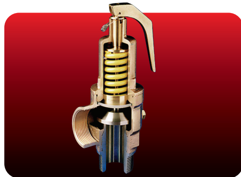
Fig. 500ST High Lift Safety Valve with Stainless Steel Wetted Parts
