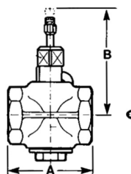
200M - Sizes 1/2" to 3"
